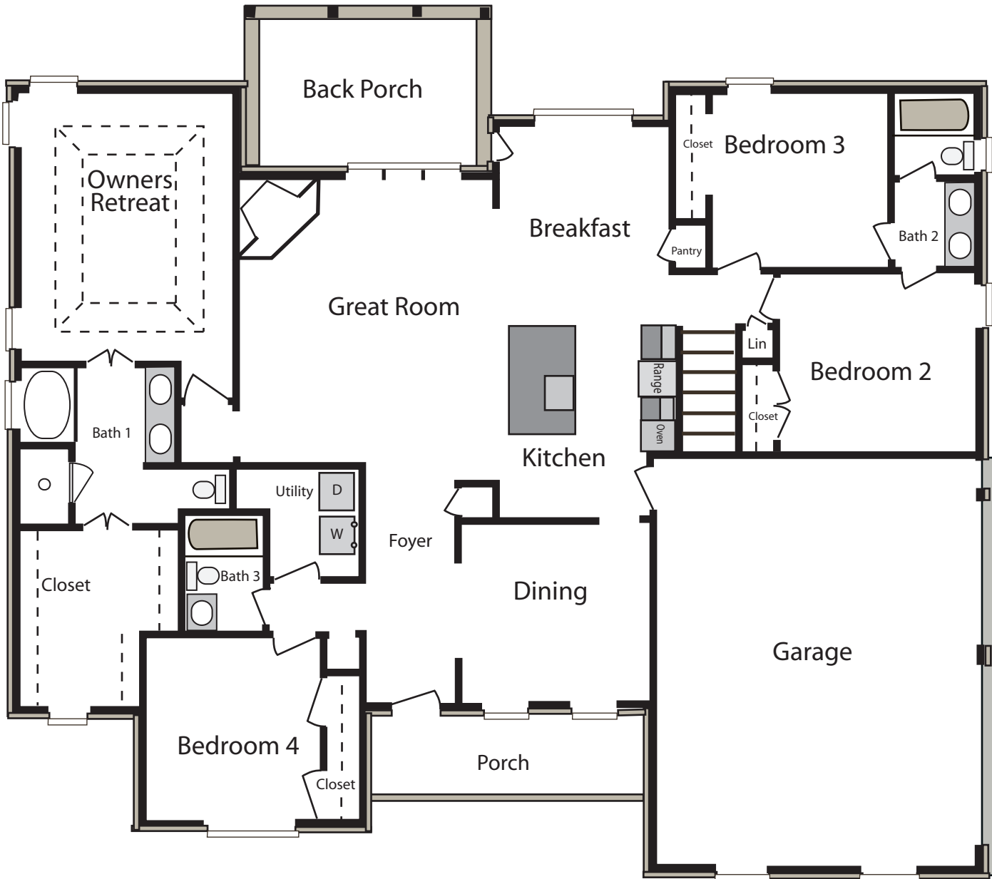
First Floor
